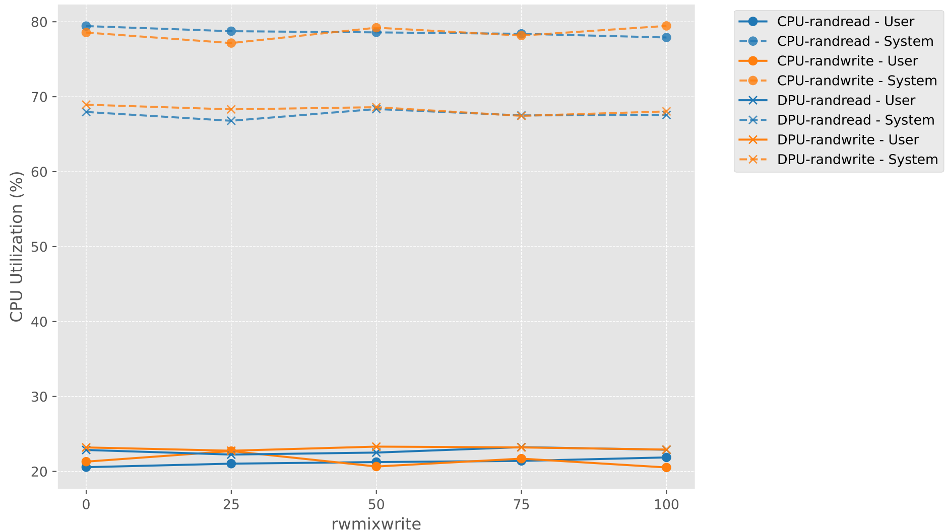
CPU Utilization vs rwmixwrite
